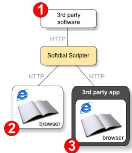
Fig. 3 - Scriptor in legacy environments
